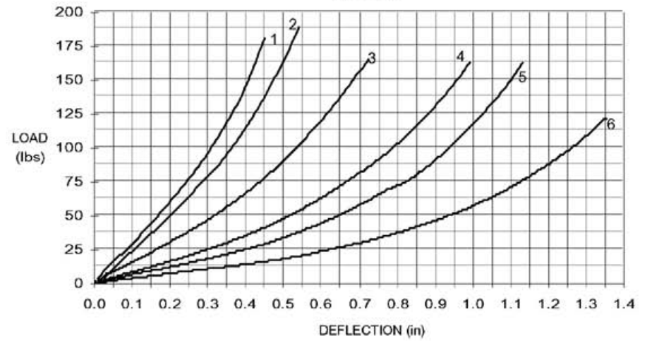
SHEAR
