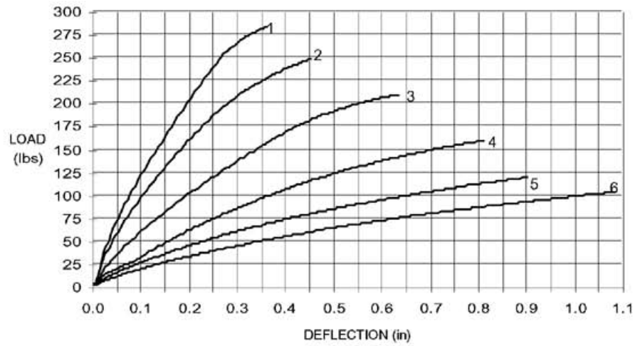
COMPRESSION
