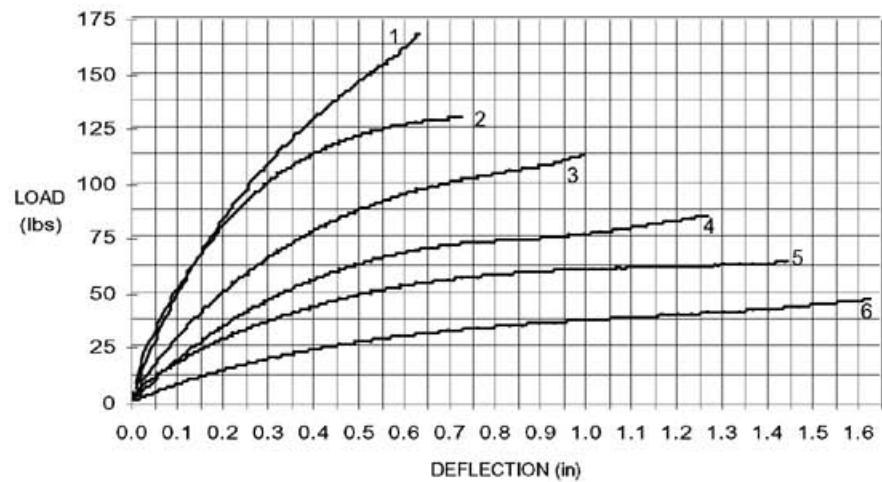
45° COMPRESSION/ROLL
