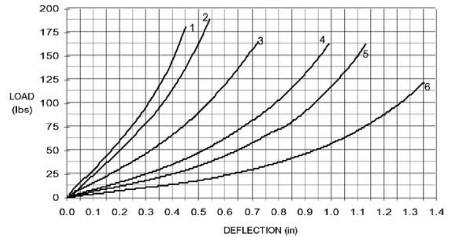
SHEAR
