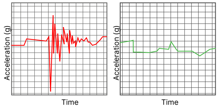
Input Shock versus Damping
