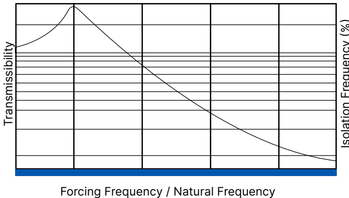
Transmissibility versus Frequency
